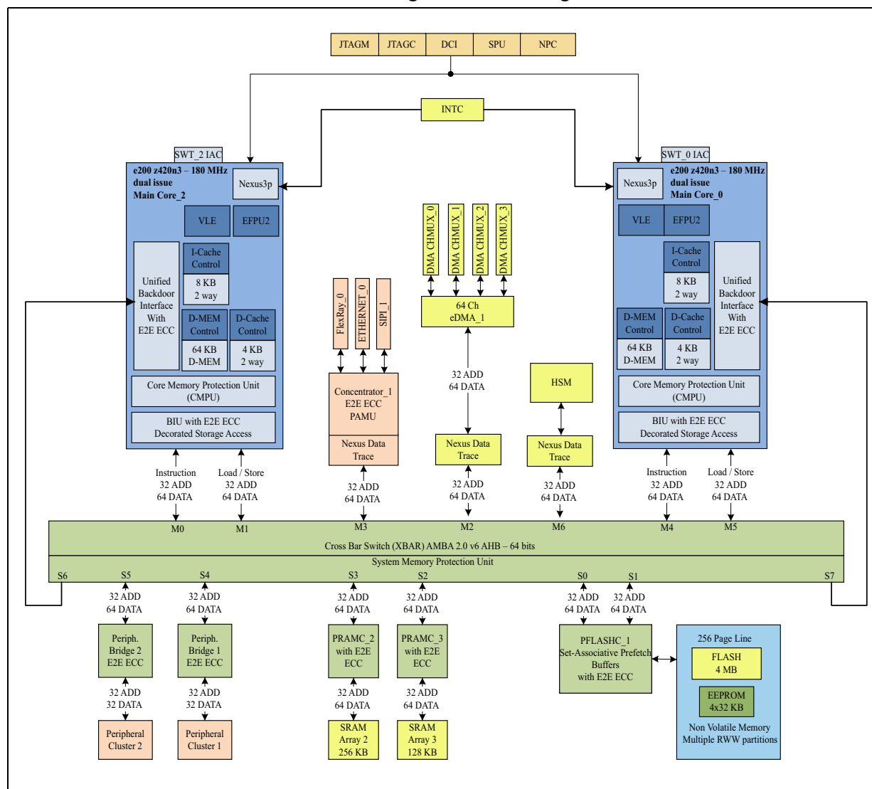
Figure 1. Block diagram
